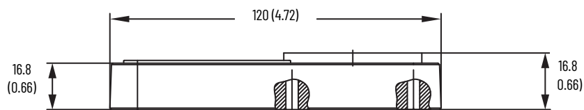
Figure 27 - Actuator [mm (in.)]
