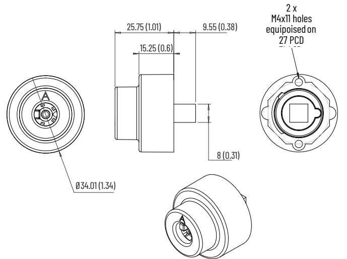
Figure 186 - 440T-MSGAU23x [mm (in.)]
