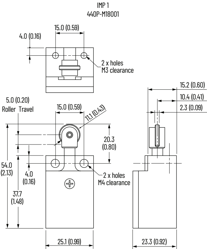
Figure 56 - Switch Body [mm (in.)]
