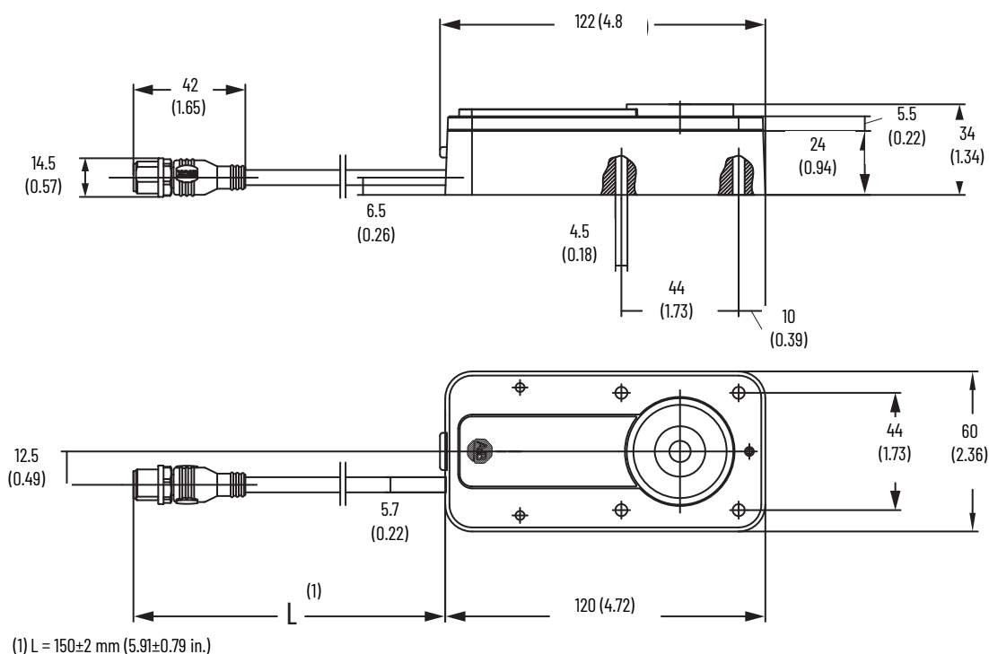
Figure 28 - Sensor [mm (in.)]
