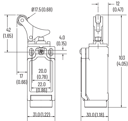
Figure 114 - Offset Hinge [mm (in.)]
