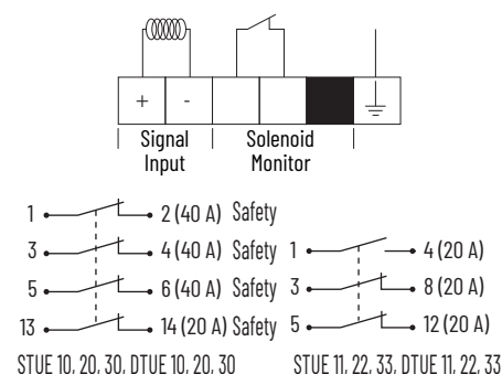
Figure 150 - Wiring (Shown with Power On)
