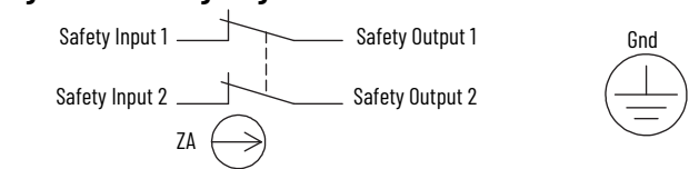
Figure 102 - Contact Opening Characteristics Plunger Type
