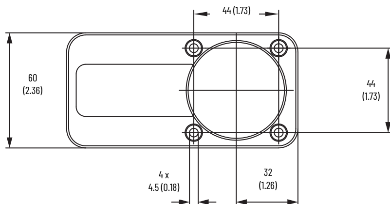
Figure 28 - Sensor [mm (in.)]
